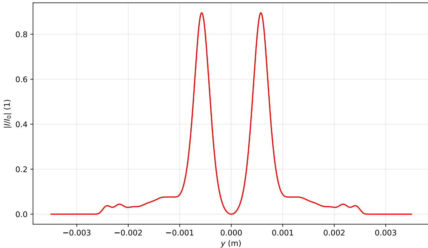
Intensity profile I(x=0, y, z=2.309)/I_0 , P_{in}=6.0P_{cr} , artificial time
